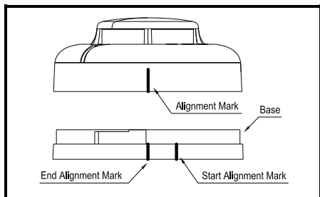
FIGURE2 Mating Detector Head onto Base
