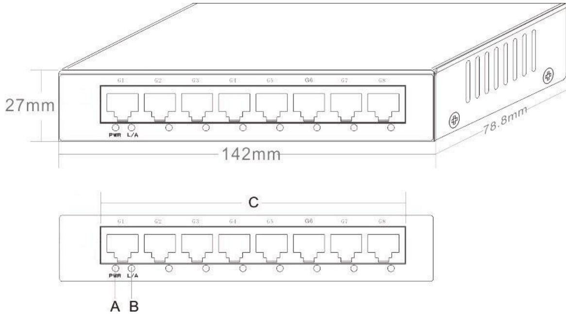
A. PWR Led Indicator B. LINK/ACT Led Indicator C. 8*10/100/100M RJ45 Ports
