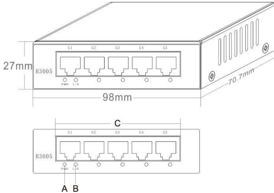
A. PWR Led Indicator B. LINK/ACT Led Indicator C. 5*10/100/1000M RJ45 Ports
