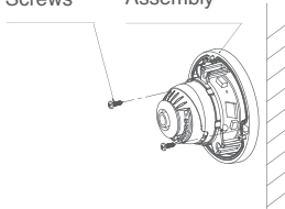
Chassis Screws
