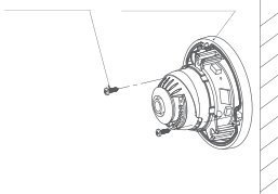
Chassis Screws
