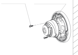
Chassis Screws
