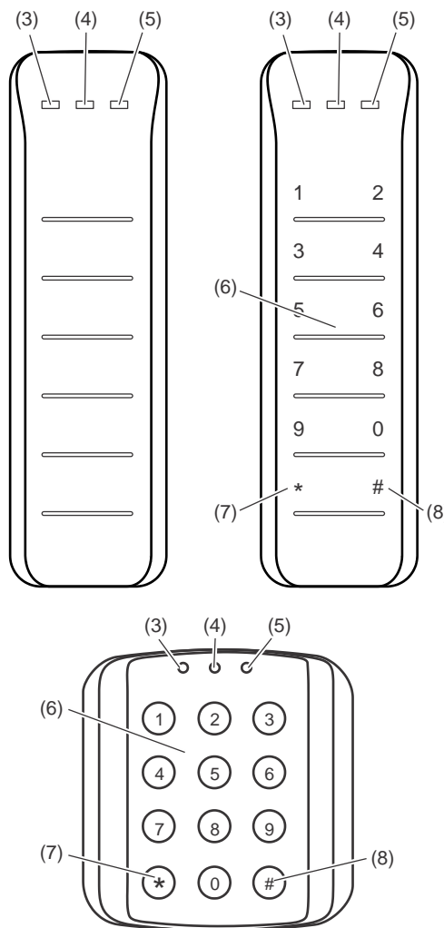
Figure 3: ATS118x readers
