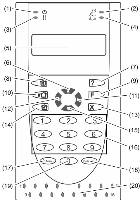
Figure 1: AT5111xA keypad
