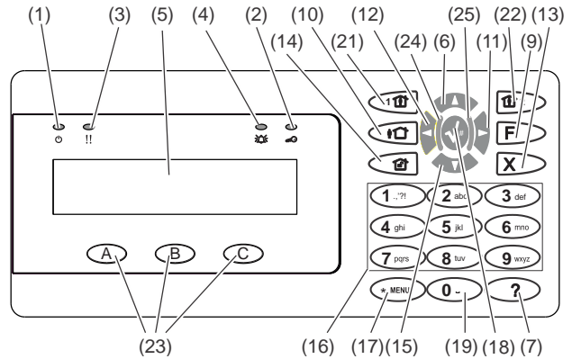
Figure 2: AT5113x keypad
